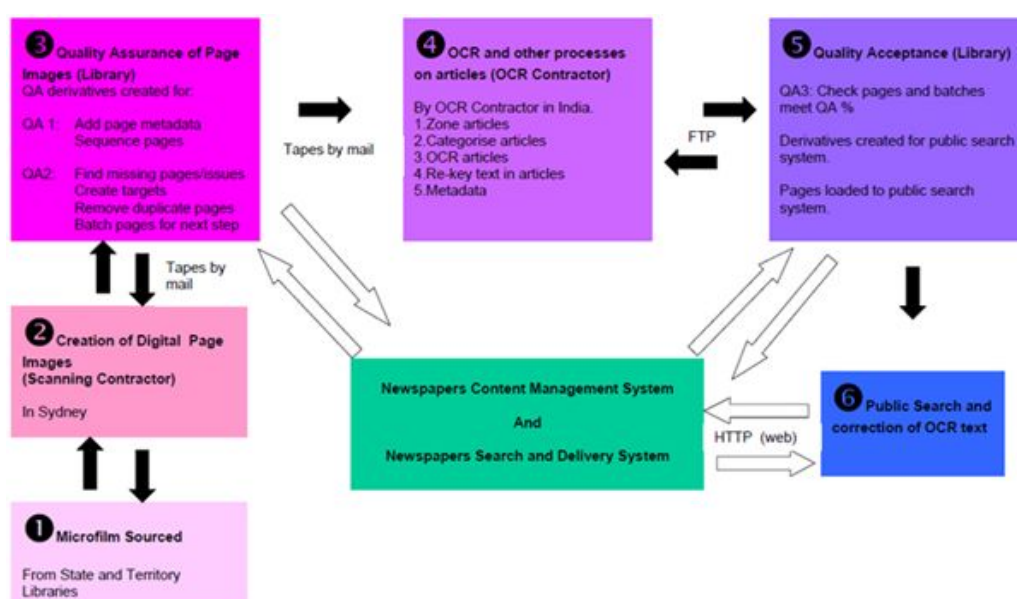
Figure 20. Trove digitisation process 2
