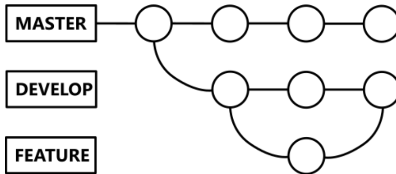
Figure 4. Git workflow: Developer and feature branches
